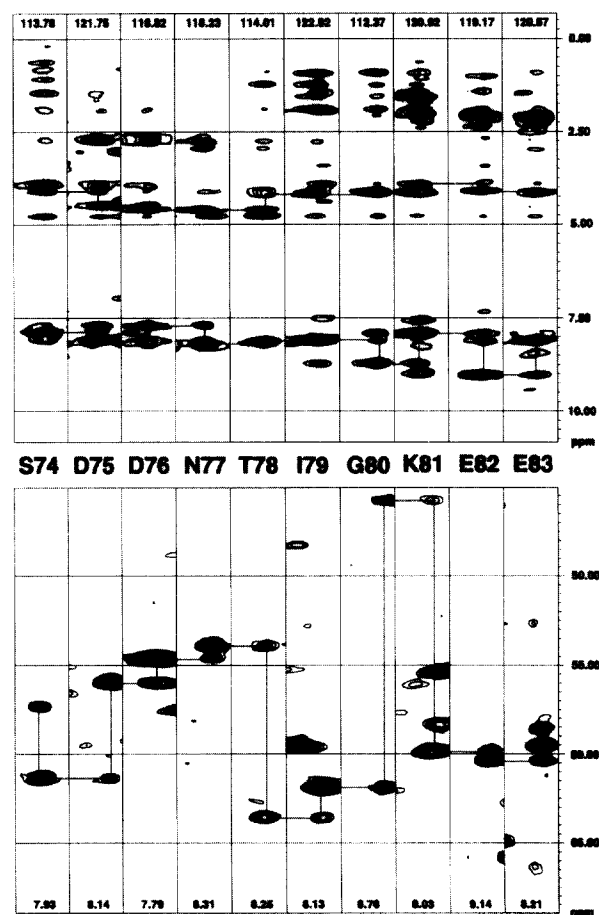
Fig. 2. ^1\text{H} - ^1\text{H} and ^1\text{H} - ^{13}\text{C} planes extracted from the 3D ^{15}\text{N} NOESY-HSQC (upper panel) and HNCA (lower panel), respectively. The ^{15}\text{N} resonance values are given at the top of each strip and the ^1\text{H} ones at the bottom (both in ppm). Shown are the ^1\text{H} - ^1\text{H} and ^1\text{H} - ^{13}\text{C} correlations for the ^{15}\text{N} edited NOESY, and the ^{13}\text{C}\alpha - ^1\text{H} correlations for the HNCA corresponding to the region around the BC loop (from Asp-76 to Gly-80).
